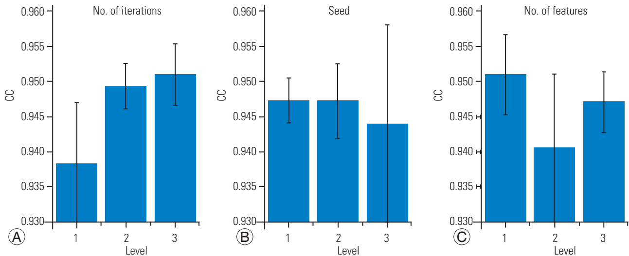
Fig. 2. (A) Variation of CC with the number of iterations. (B) Variation of CC with seed. (C) Variation of CC with the number of features. CC, correlation coefficient.
